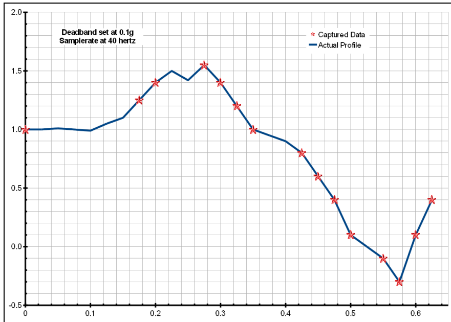
Figure 3: Graphical Illustration of the Deadband Feature
