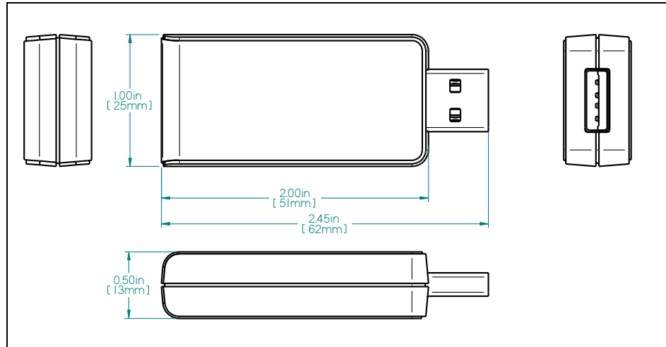
Figure 9: Enclosure Dimensions
