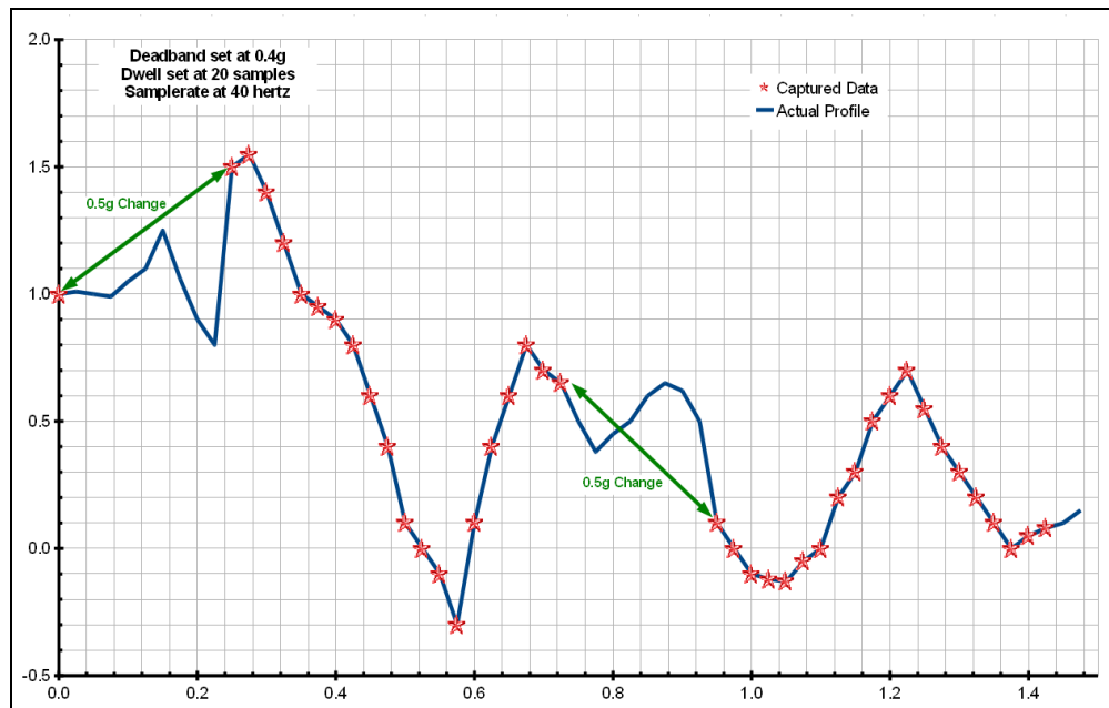
Figure 4: Graphical Illustration of the Dwell Feature
